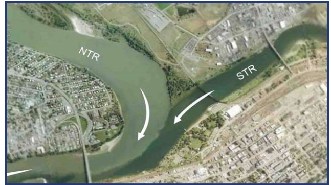
Figure 21. A satellite image of the confluence of the silty grey North Thompson River (upper left) and clear blue-green South Thompson River (right) to form the Thompson River (lower left). The Overlander Park sand and gravel bar is visible at the confluence. Photo courtesy of Google Earth.
